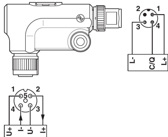
Figure 6 4-conductor connection example
