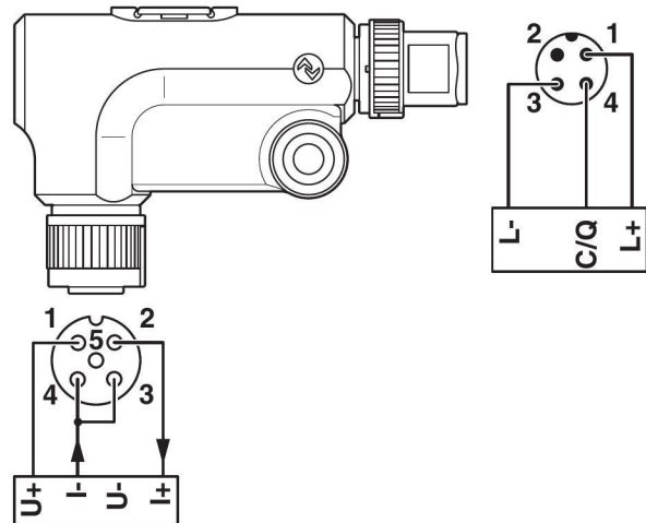
Figure 5 3-conductor connection example
